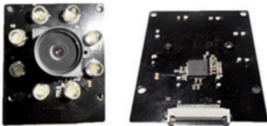
HDF9712-LED L*W:38*38mm
